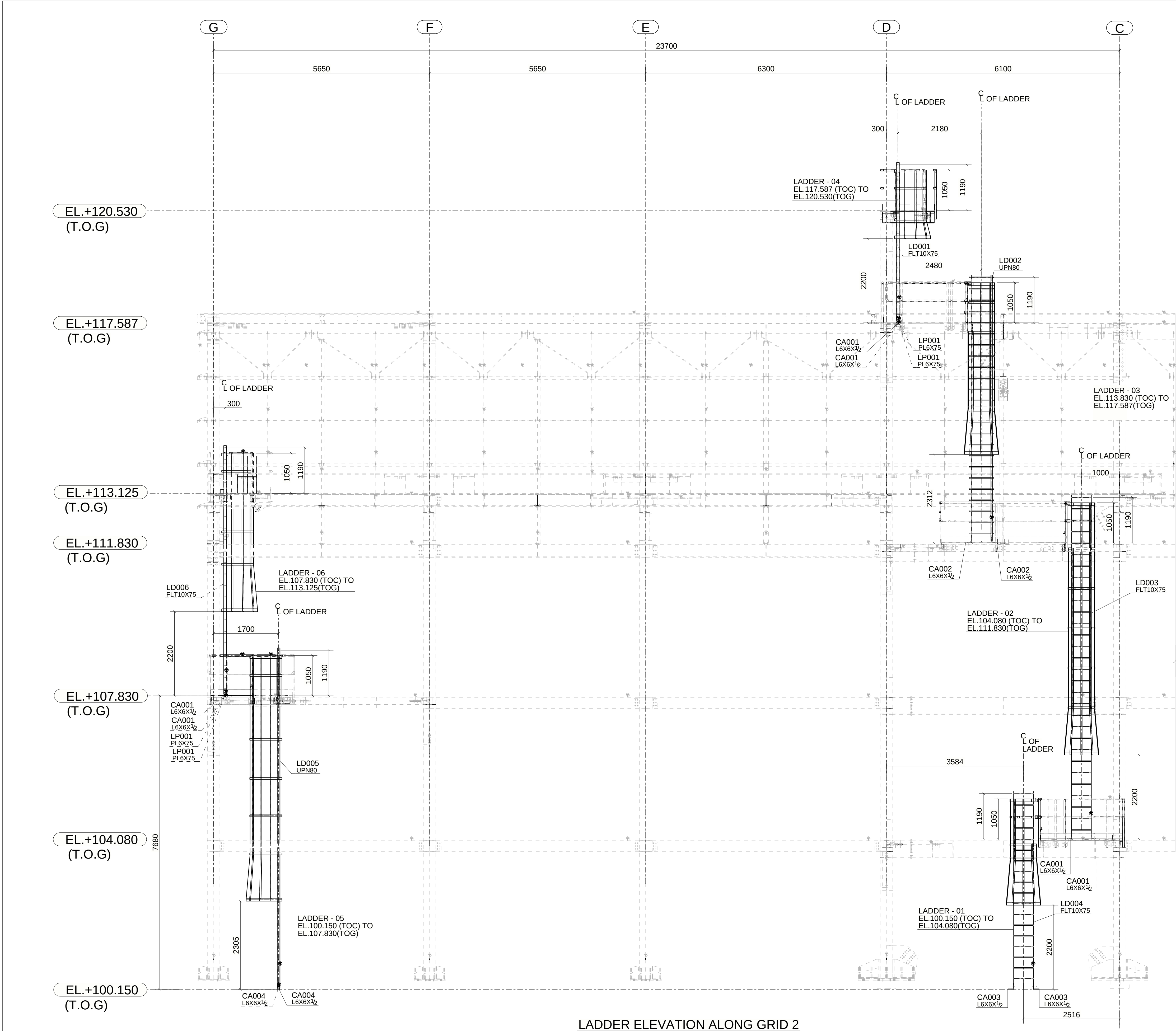
LADDER ELEVATION ALONG GRID 2
