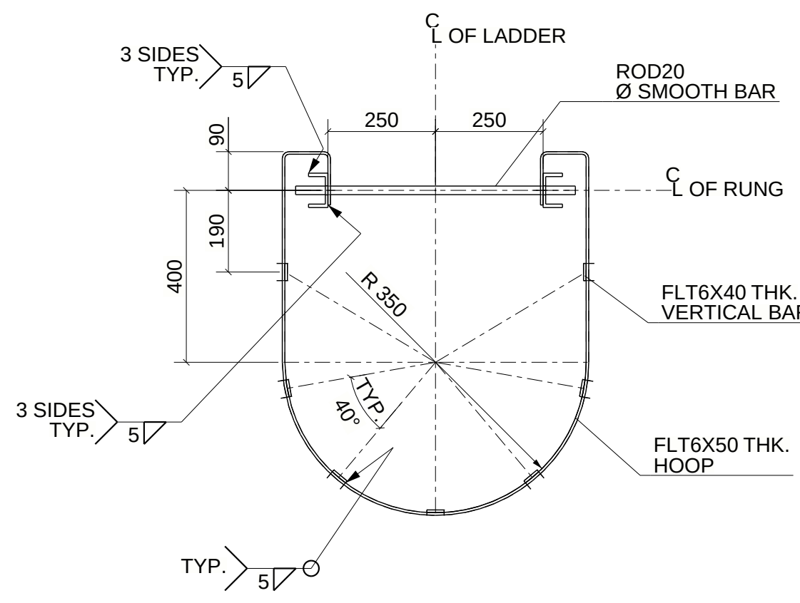
SECTION - 1T - 1T
