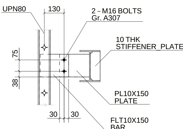
DETAIL - 12
