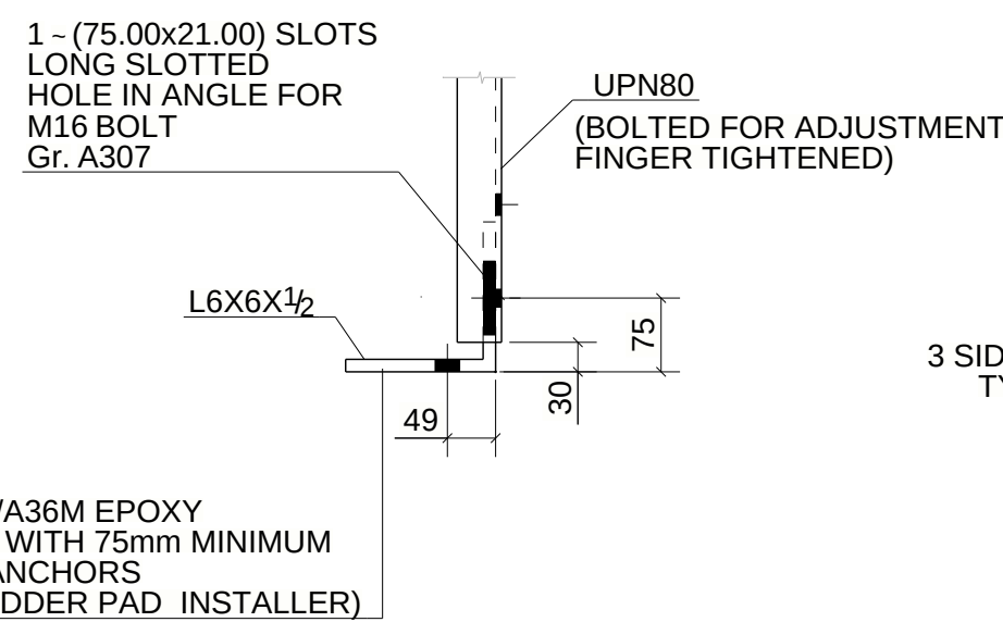
DETAIL - 10
