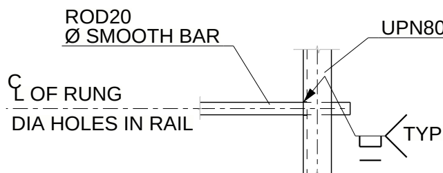
DETAIL - 11
