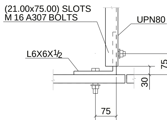
TYPICAL LADDER TO GRATING CONNECTION
