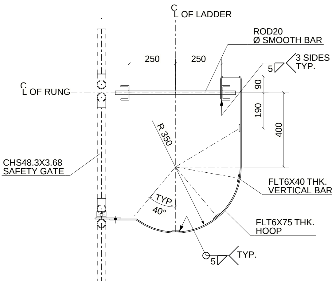
SECTION - 1U - 1U
