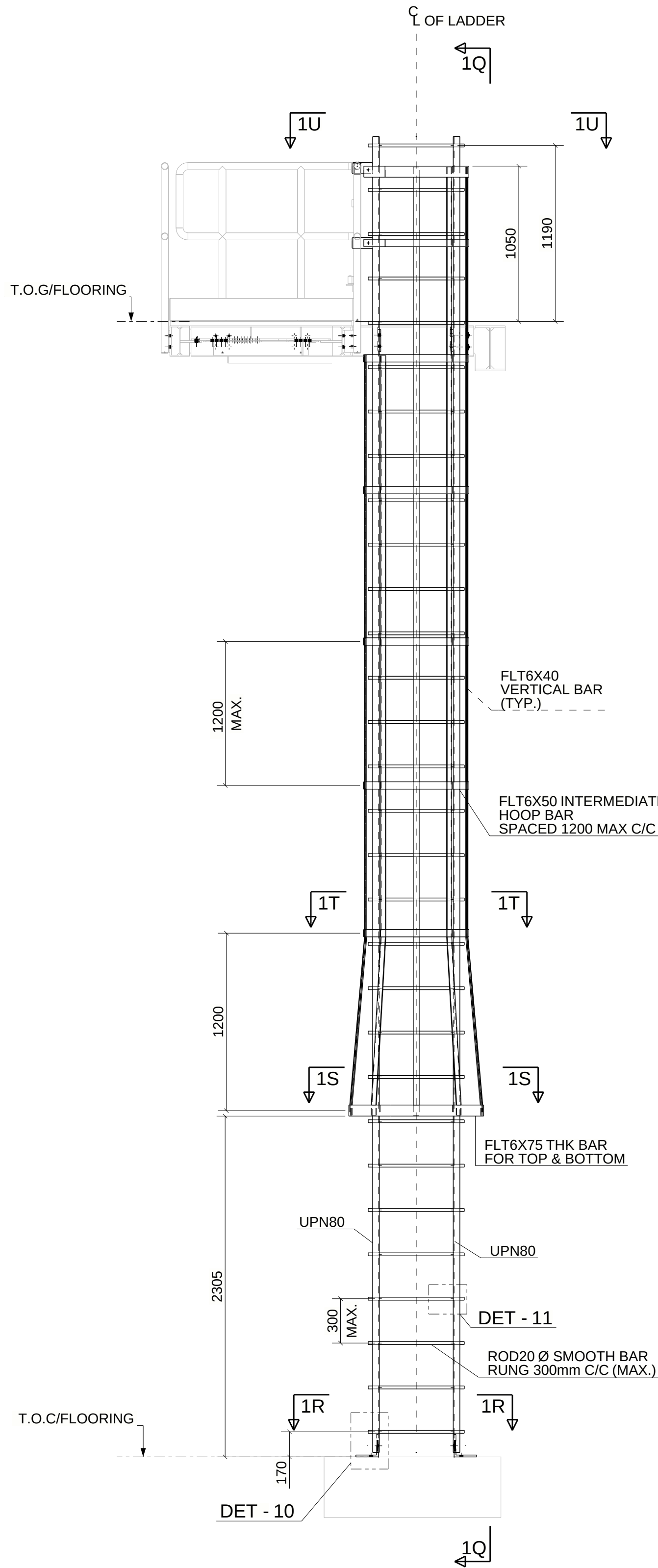
TYPICAL LADDER DETAIL
